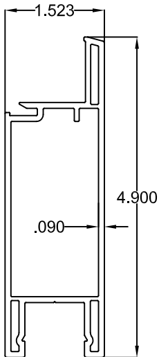
7 PANEL STILE/RAIL
