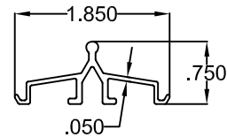
12 ROLLER TRACK
