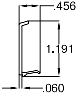
3 GLAZING BEAD
