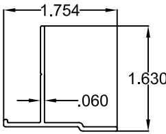
22 HOOKSTRIP FLANGE
