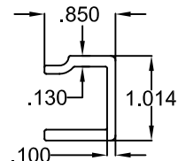
26 REINF. MULLION
